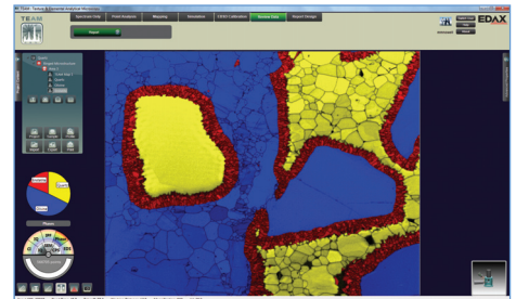
EBSD Image Quality and Phase map of olivine (blue), quartz (yellow), and enstatite (red).
