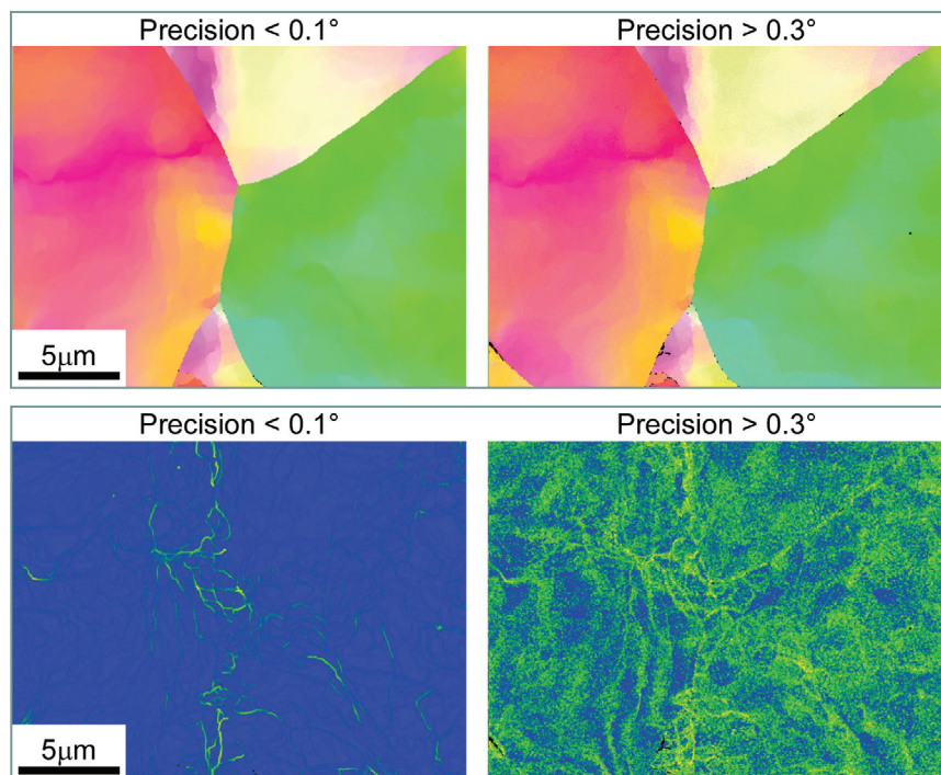
Orientation maps (top) and kernel average misorientation (KAM) maps from a deformed steel sample. The orientation maps suggest there is little difference in the measurements. However, the KAM maps with orientation precision values less than 0.1 degrees show that the deformation structure is sharply defined by local increases in KAM values, while with precision values greater than 0.3 degrees, this detail is lost due to higher noise in the measurements.
