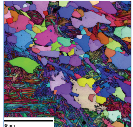
Orientation map from dual phase low carbon steel. DigiView provides high indexing rates from both phases for results without compromise.
